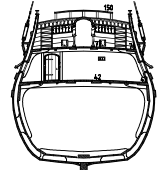
Frame 27
