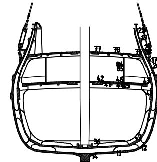
Frame 13
