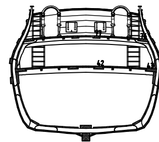
Frame H
