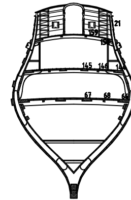
Frame 40
