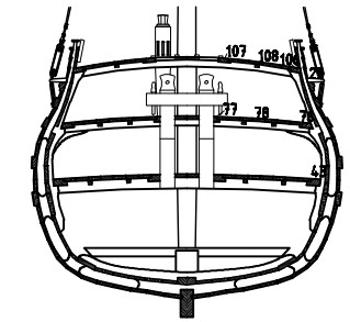
Frame R
