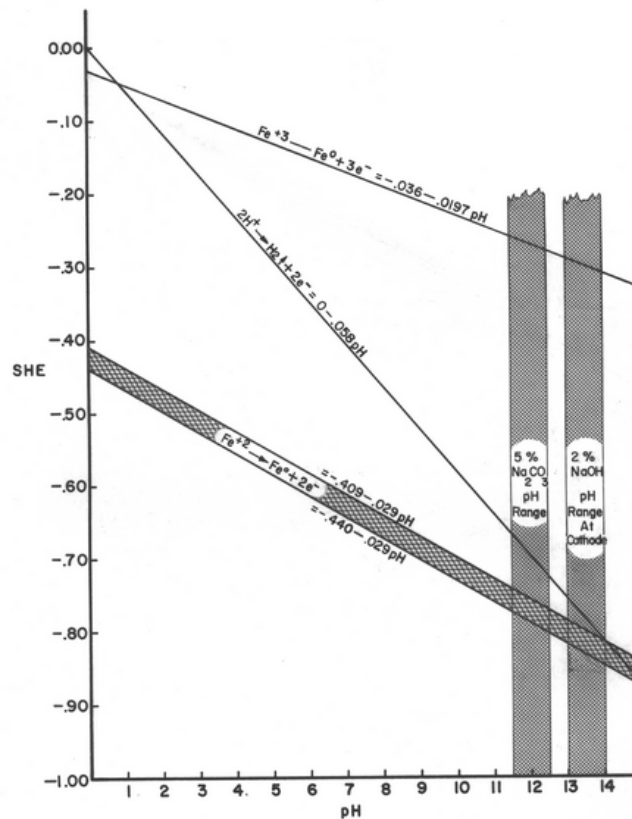
Figure 10B.3. Reduction potentials of ferric, ferrous, and hydrogen ions at different pHs and standard temperature of 20°C. The pH range of a 5 percent \text{Na}_2\text{CO}_3 and a 2 percent \text{NaOH} electrolyte are shaded.
