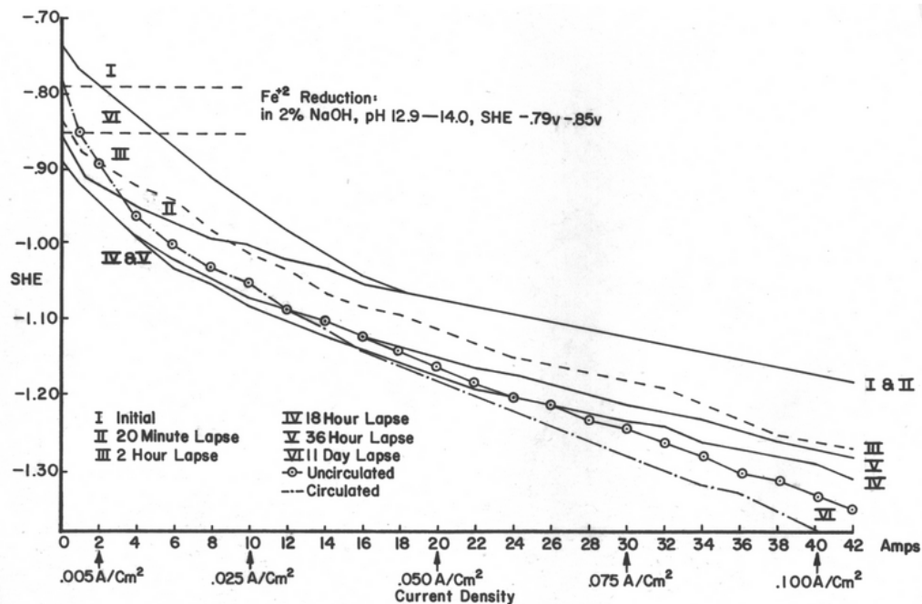
Figure 10B.4. Reduction potentials at the surface of an iron cathode during electrolysis in a 2 percent NaOH electrolyte at different current densities over an 11-day test period.
