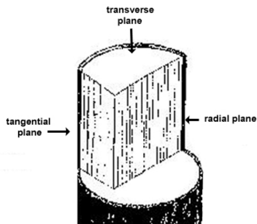
Figure 6.3 . Schematic drawing, illustrating the three principal planes in wood: transverse, tangential, and radial.
