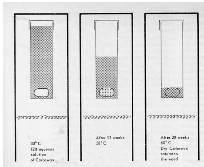
Figure 6.5. Setup for treatment of small specimens of waterlogged wood.
