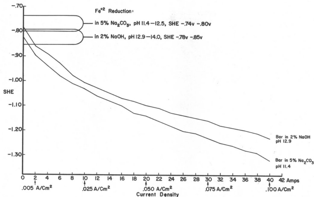
Figure 10B.5. Comparison of the reduction electrode potential on the surface of the same iron cathode in a 5 percent \text{Na}_2\text{CO}_3 and a 2 percent NaOH electrolyte.
