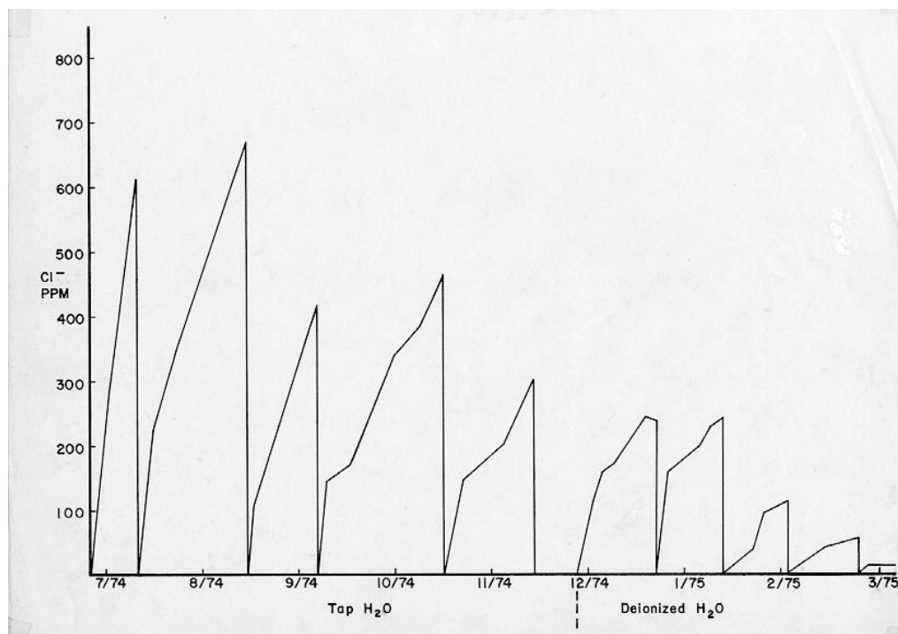
Figure 10A.2 . Graph depicting the diffusion of chlorides into solution during electrolysis.
