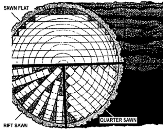
Figure 6.4. Methods of sawing logs for lumber: flat-sawn, rift-sawn, and quarter-sawn.
