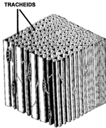
Figure 6.2 . Schematic diagram of softwood, illustrating the relative appearance of tracheids.
