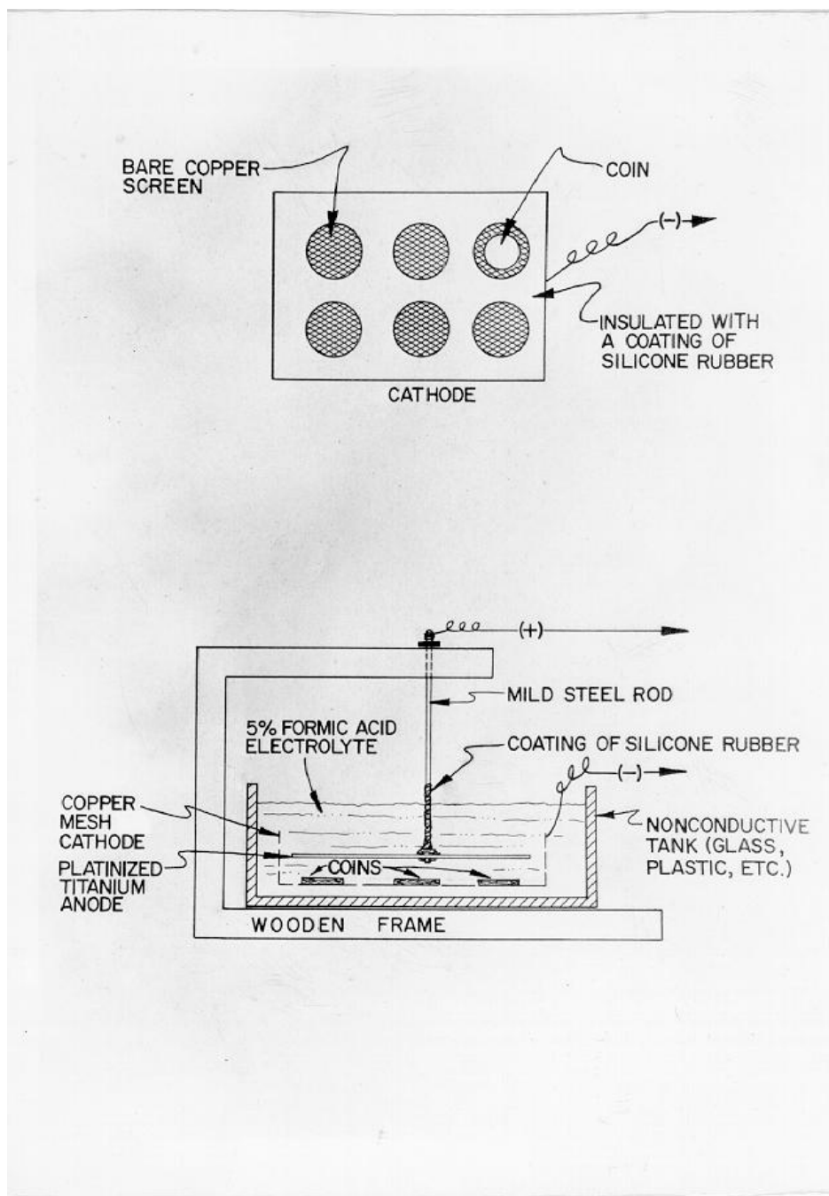
Figure 13.1. Electrolytic setup for cleaning silver coins or other small artifacts.
