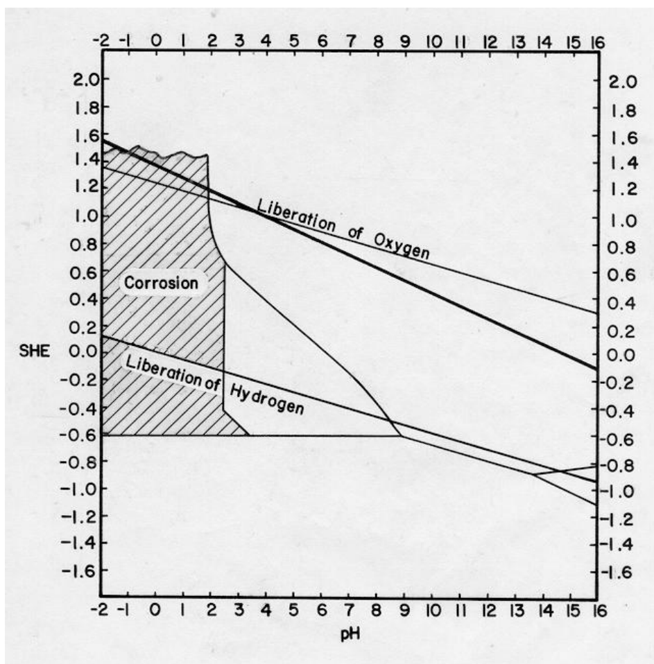
Figure 9.1 . Stability conditions of pure iron in a chromate solution.
